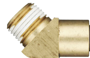
27196 Male Elbow 45° 3/8 Tube x 1/4 NPT
